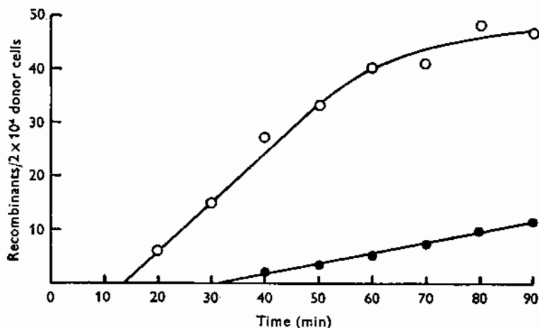
Fig. 3. Time of entry kinetics of ilvA12 and his-2 markers (OT15 str a × OT92 ilvA12 his-2 str r ). The cells were diluted in nitrate NB after 20 min pairing. Samples for plating were removed from the diluted cells. ○, ilvA12 ; ●, his-2 + .
