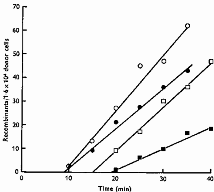
Fig. 4. The effect of dilution on the time of entry kinetics of ilvA12 and his-6 markers (OT15 str a × OT101 ilvA12 his-6 leu-1 str r ). Pairing was restricted to 5 min when the cells were diluted in nitrate NB. Samples for plating were removed from these diluted cells as well as from the original undiluted material. This latter sample was diluted prior to plating. ○, ilvA12 + diluted 10 -3 at 5 min; ●, ilvA12 + diluted at sampling; □, his-6 + diluted 10 -3 at 5 min; ■, his-6 + diluted at sampling.
