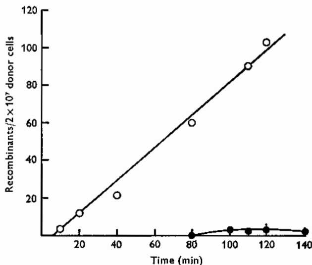
Fig. 1. Time of entry kinetics of lys-1 and leu-1 markers (OT15 str s × OT10 lys-1 leu-1 str r ). Pairing was unrestricted and cells were plated without dilution after mating had been interrupted on a Mickle shaker. ○, lys-1 + ; ●, leu-1 + .
